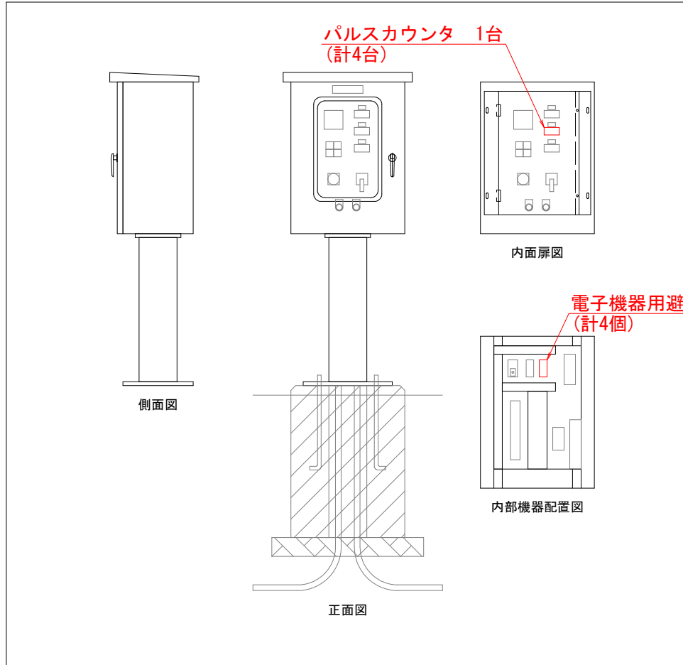
機器配置図 (No. 4, No. 8, No. 11, No. 13)
