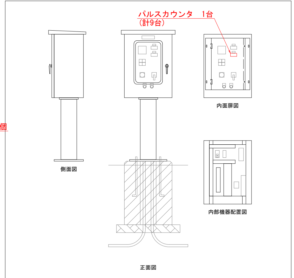
機器配置図 (No. 1, No. 2, No. 3, No. 5, No. 6, No. 7, No. 9, No. 10, No. 12)
